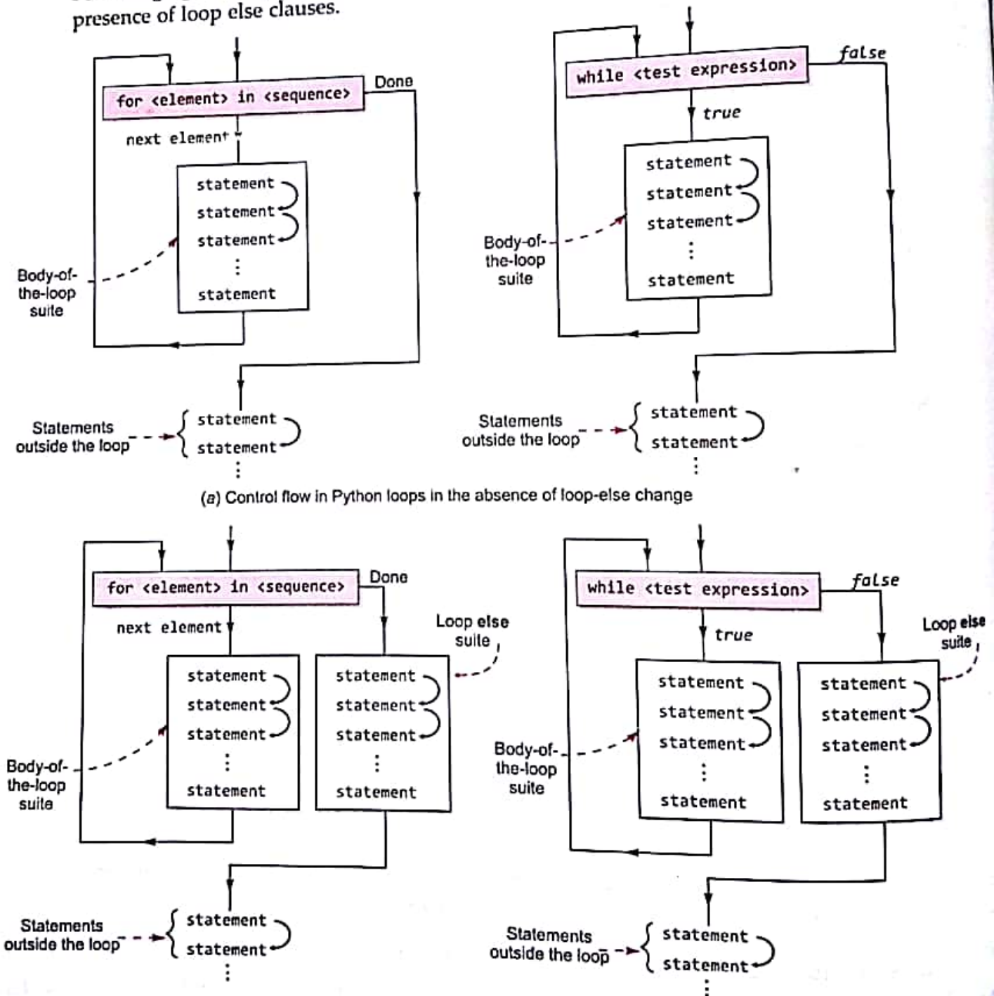
(b) Control flow in Python loops in the presence of loop-else clause.
